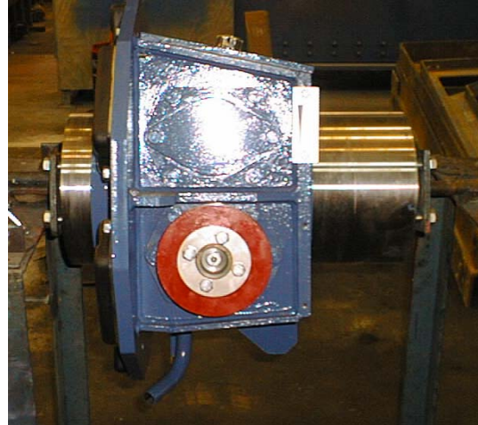
Assembled Vibrator Unit prior to fitting in HSG 1100 centrifuge.
