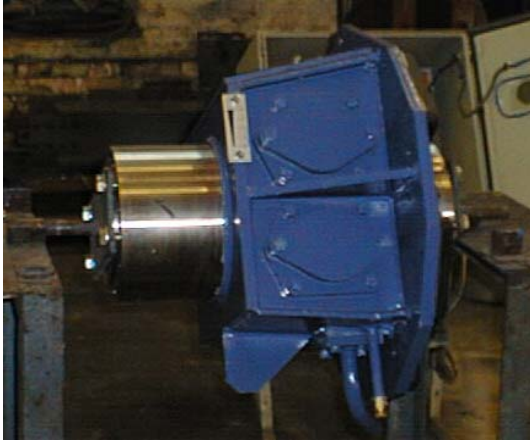
Assembled Vibrator Unit prior to fitting in HSG 1100 centrifuge.
