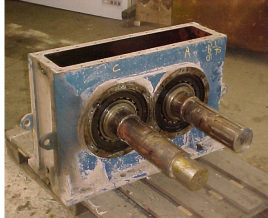
Exciter Unit Prior to Refurbishment
